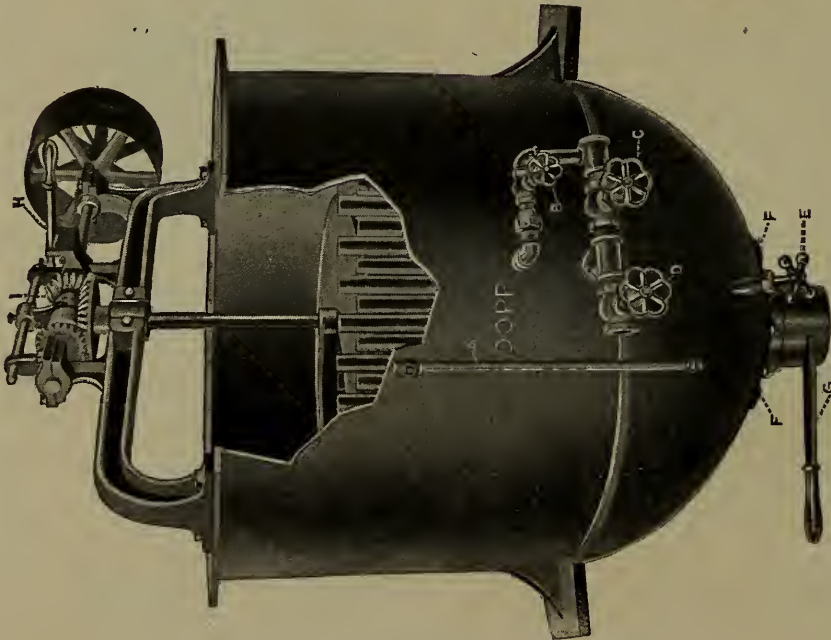
STYLE "A"—BELT-DRIVEN
